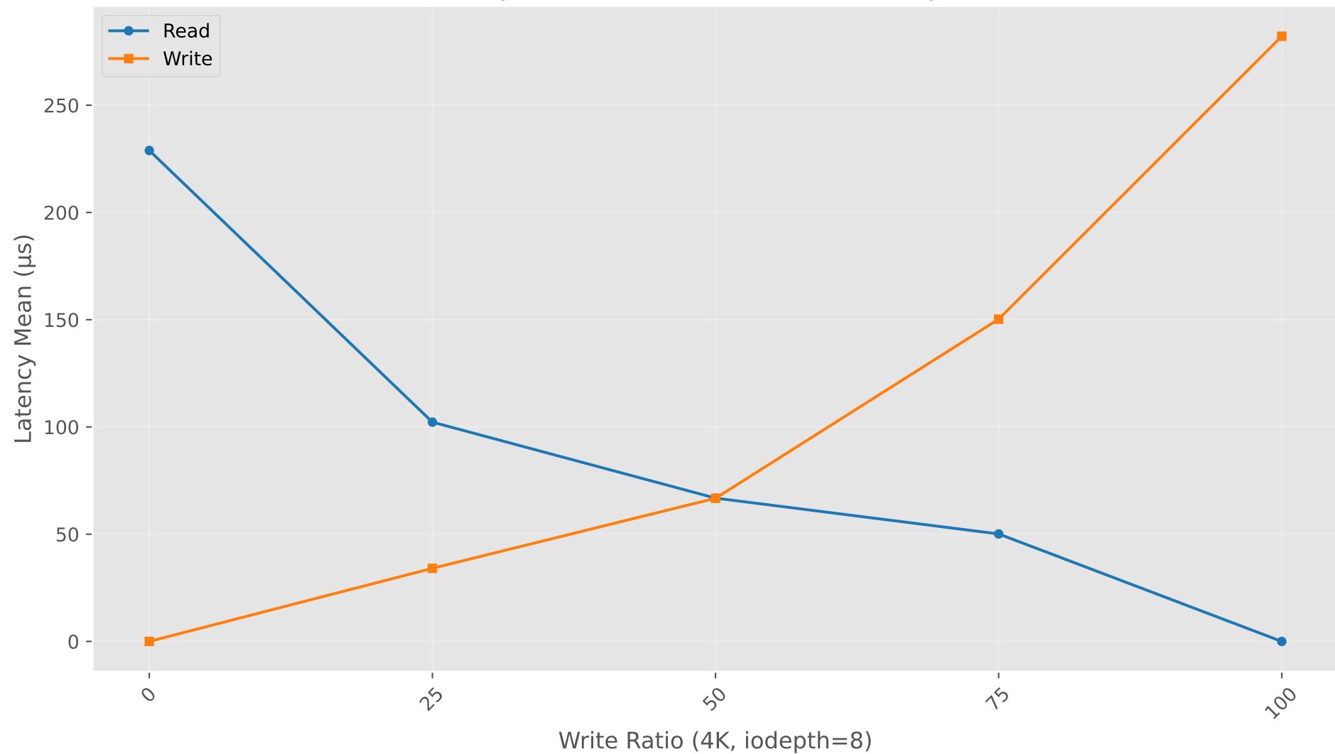
Latency Mean vs Write Ratio (4K, iodepth=8)
